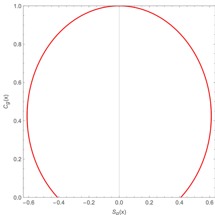
Figure 1. Gaussian trigonometric “circumference”: egg-shaped curve. C_g(x) vs. S_g(x) .
