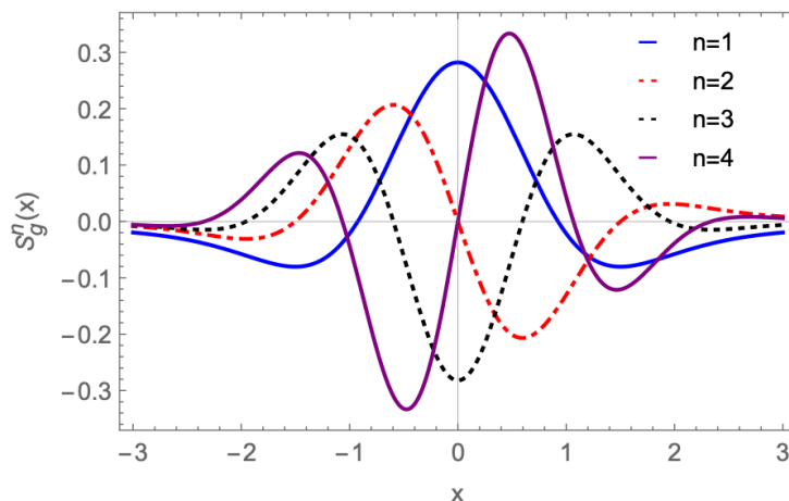
Figure 3. Normalized S_g^{(n)}(x) for different values of n .
