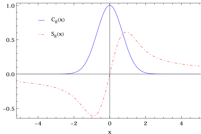
Figure 2. C_g(x) and S_g(x) vs. x .
