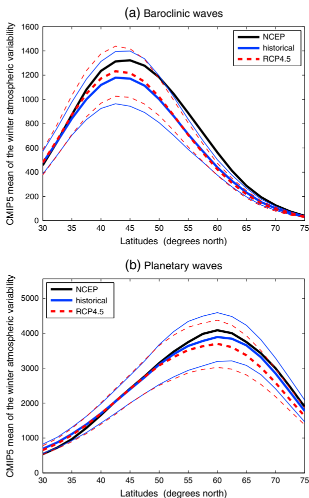
Figure 3. Meridional profiles in the belt 30°N–75°N of (a) \langle E_{\text{Baroc}} \rangle of the baroclinic waves and (b) \langle E_{\text{Plan}} \rangle of the planetary waves, averaged on the CMIP5 models for the 1979–2001 historical simulations (blue solid lines), compared with the NCEP reanalysis on the same years (black line), and the 2058–2080 RCP4.5 simulations (red broken lines). In Figures 3a and 3b, for historical and RCP4.5 simulations, the heavy lines represent the mean and the thin lines delimit the variance of the CMIP5 ensemble.
