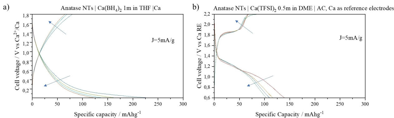
Figure 4. Performance of the a-NTs electrodes by using the C1 or C2 cell configurations. Current rate 5 \text{mA g}^{-1} ; shown cycles are 2–5 of the whole galvanostatic test and are obtained after 1 activation cycle.
