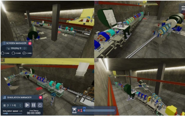
Figure 29. Operator view of the RH operation through the viewing system in VR simulations. Reproduced from [17]. CC BY 4.0.
