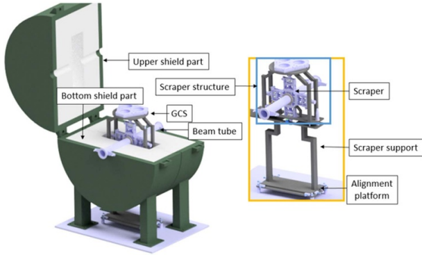
Figure 15. Structure of the HEBT scraper [10, 12].
