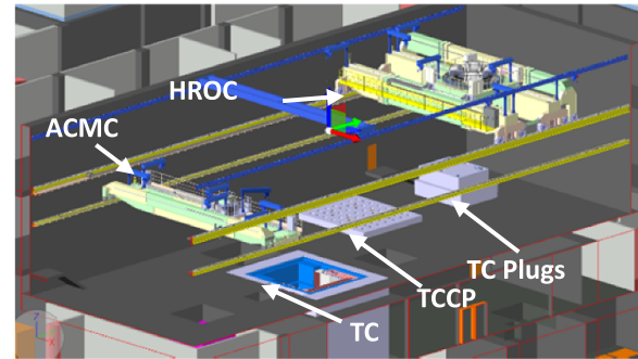
Figure 4. View of the AC and cranes for TC maintenance.
