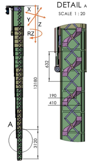
Figure 7. Fully extended boom and cables management.
