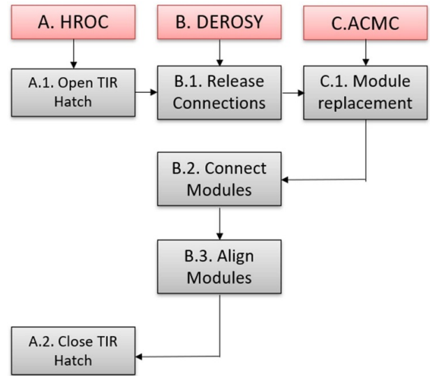
Figure 21. Flowchart for TIR module replacement.
