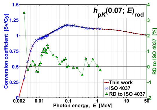
Figure C4. Values for h_{pK}(0.07; E)_{rod} for the rod phantom calculated in this study, h_{MC} (red line), published in ISO 4037–3:2019, h_{ISO} (blue crosses), and their relative difference, RD = h_{MC}/h_{ISO} - 1 , at energies where values of both data sets were available (triangles, right axis).
