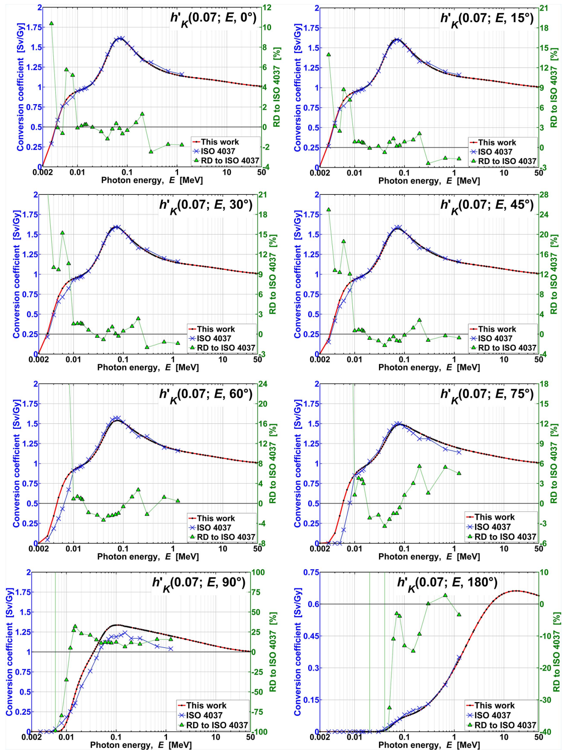
Figure C1. Values for h'_K(0.07; E, \alpha) for various angles of radiation incidence, \alpha , calculated in this study, h_{MC} (red line), published in ISO 4037–3:2019, h_{ISO} (blue crosses), and their relative difference, RD = h_{MC}/h_{ISO} - 1 , at energies where values of both data sets were available (triangles, right axis).
