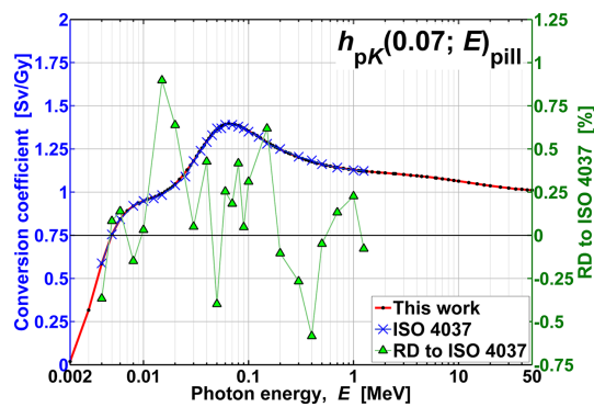
Figure C5. Values for h_{pK}(0.07; E)_{pill} for the pillar phantom calculated in this study, h_{MC} (red line), published in ISO 4037–3:2019, h_{ISO} (blue crosses), and their relative difference, RD = h_{MC}/h_{ISO} - 1 , at energies where values of both data sets were available (triangles, right axis).
