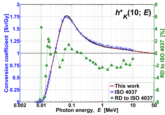
Figure C3. Values for h_K^*(10; E) calculated in this study, h_{MC} (red line), published in ISO 4037–3:2019, h_{ISO} (blue crosses), and their relative difference, RD = h_{MC}/h_{ISO} - 1 , at energies where values of both data sets were available (triangles, right axis).
