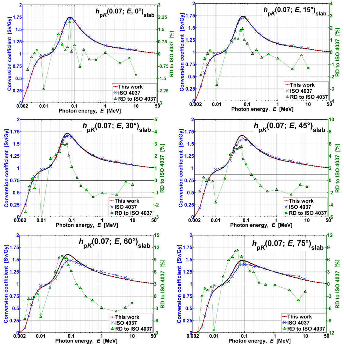
Figure C6. Values for h_{pK}(0.07; E, \alpha)_{\text{slab}} for the slab phantom for various angles of radiation incidence, \alpha , calculated in this study, h_{MC} (red line), published in ISO 4037–3:2019, h_{ISO} (blue crosses), and their relative difference, RD = h_{MC}/h_{ISO} - 1 , at energies where values of both data sets were available (triangles, right axis).
