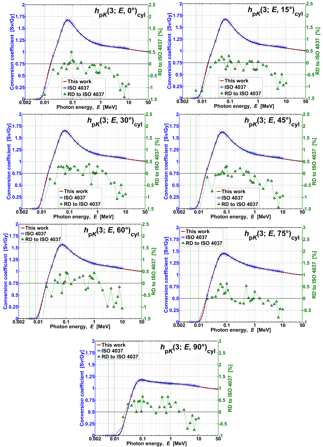
Figure C7. Values for h_{pK}(3; E, \alpha)_{\text{cyl}} for the cylinder phantom for various angles of radiation incidence, \alpha , calculated in this study, h_{MC} (red line), published in ISO 4037–3:2019, h_{ISO} (blue crosses), and their relative difference, RD = h_{MC}/h_{ISO} - 1 , at energies where values of both data sets were available (triangles, right axis).
