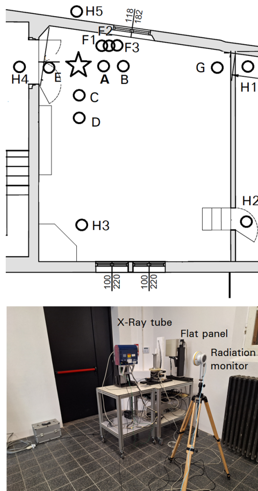
Figure 2. The scheme of the measuring (A)–(G) and simulation points (A)–(G) and (H1–H5) (top); the equipment employed for the tomography and the radiation monitor placed in position A (bottom).
