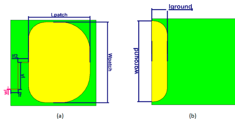
Figure 7. Configuration of the proposed antenna: (a) Top view; (b) Bottom view.
