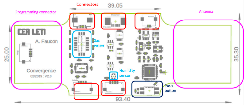
Figure 6. Flex PCB: design and dimensions.
