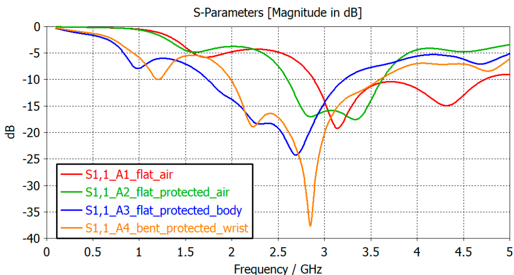
Figure 4. Simulated reflection coefficient of the proposed antenna in four scenarios: A1 placed in air; A2 protected by varnish and silicon; A3 placed on human body; A4 bent on human’s wrist.
