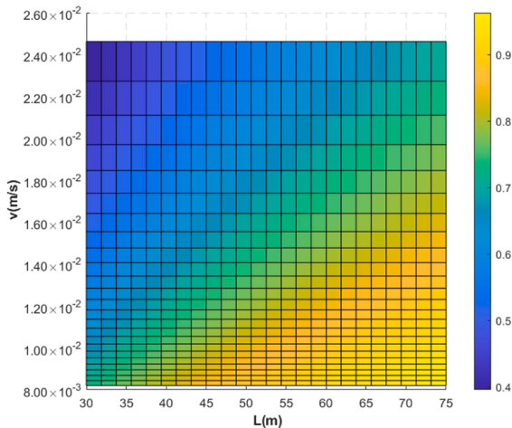
Fig. 6. Vanadium-plate-PAV efficiency as a function of PbLi velocity and membrane length. [width = 1.4 m; channel height 5 \cdot 10^{-3} m; membrane thickness = 1 \cdot 10^{-3} m; 200 PbLi channels].
