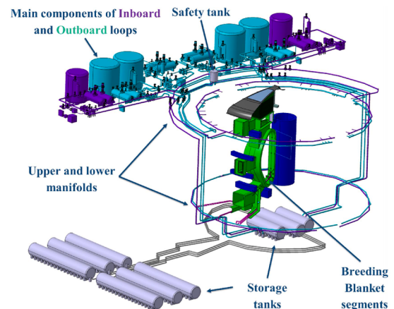
Fig. 2. 3D drawing of the WCLL TER (the OB loops are colored in teal, the IB loops in purple, shared components in grey).
