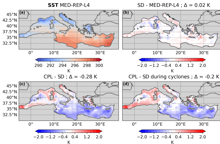
Figure 6. Same as Fig. 5 but for SON.
