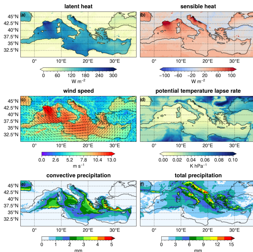
Figure 4. Maps for latent heat flux (a), sensible heat flux (b), 10 m wind speed and direction (c), potential temperature lapse rate (d), convective precipitation (e), and total (large-scale + convective) precipitation (f) from the STD simulation during extreme winter cyclones in common with CPL.
