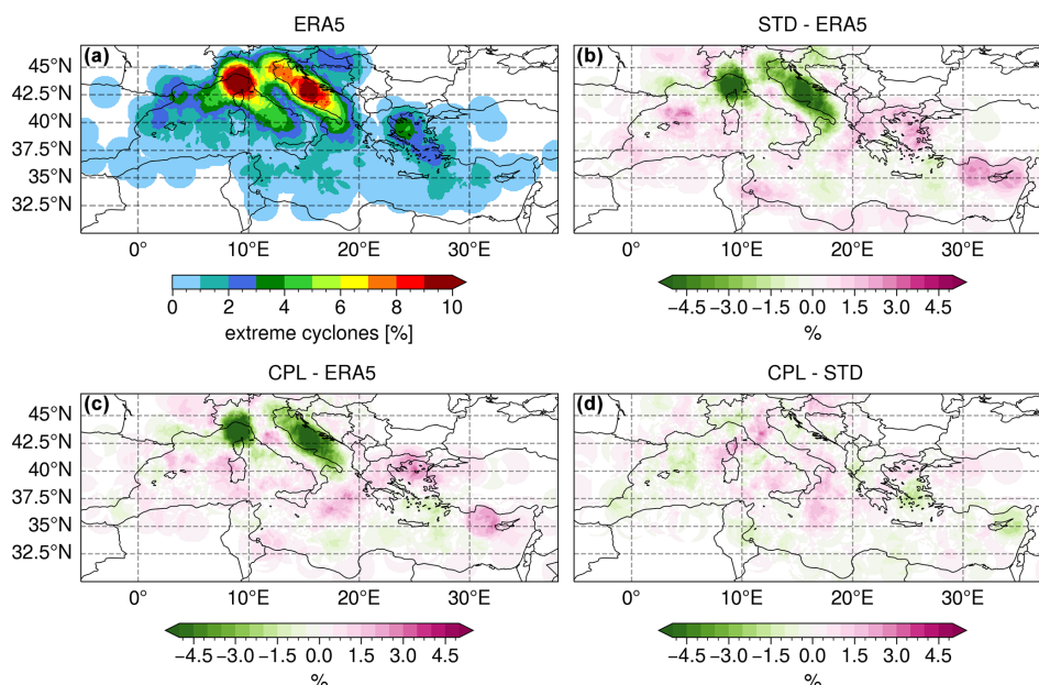
Figure 3. Cyclone centre densities (CCDs) for the 500 most intense cyclones in ERA5 (a), along with CCD differences between STD and ERA5 (b), CPL and ERA5 (c), and CPL and STD (d). The values are normalised by the total number of cyclones (i.e. 500) and expressed as a percentage. To highlight the cyclones' area of influence, each centre is represented by a circular area with a radius of 1.5^\circ around the tracked minimum SLP point.
