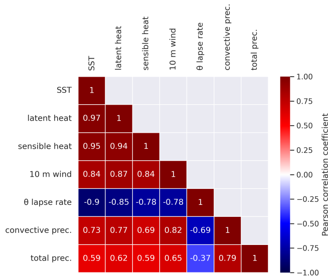
Figure 9. Pearson correlation coefficient ( R ) between the SST differences (Fig. 5b, CPL – STD) and the differences in the atmospheric fields analysed (Fig. 7, CPL – STD) during the extreme winter cyclones. The matrix is symmetric. \theta stands for potential temperature.
