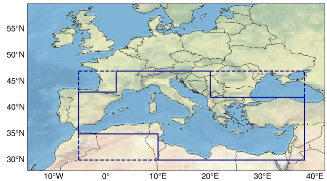
Figure 1. Med-CORDEX domain. Cyclones are retained if their minimum SLP tracking point is present within the area outlined by solid lines. The atmospheric fields are computed within the rectangular area outlined by dashed lines.
