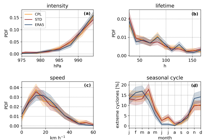
Figure 2. Statistics on intensity (a), lifetime (b) and speed (c), and seasonal cycle (d) of the 500 most intense cyclones in STD, CPL and ERA5. The colour bands represent the 2.5%–97.5% confidence interval within the 1000 bootstrap surrogates.
