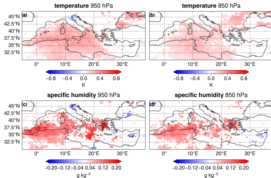
Figure 8. Maps of the differences between CPL and STD during the common extreme winter cyclones for temperature (a, b) and specific humidity (c, d) at 950 and 850 hPa. The white colour indicates no significant differences at the 5 % confidence level.
