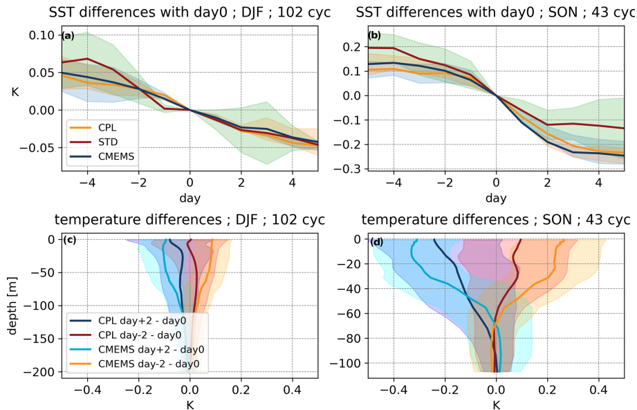
Figure 10. SST evolution compared with the SST on the day of the cyclone from 5 d before to 5 d after the event for CPL (orange line), STD (red line) and the CMEMS MED-Currents reanalysis (blue line), averaged over the same cyclones in DJF (a) and in SON (b). The vertical profiles of the ocean temperature computed as the difference between 2 d before and the day of the cyclones (similarly for 2 d after the event) for CPL (blue and red lines) and CMEMS MED-Currents (light-blue and orange lines), averaged over the same cyclones in DJF (c) and in SON (d). In each figure the temperature values represent the average over a circular area with a 1.5^\circ radius, around the minimum SLP tracking point and over the cyclones considered. The colour bands represent the confidence interval between \pm 1 standard deviation of the mean of the temperature differences.
