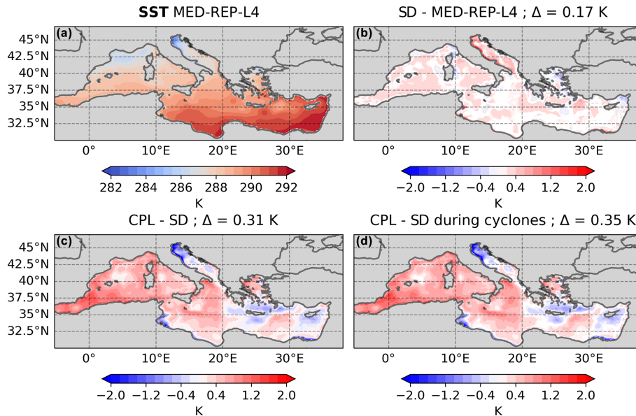
Figure 5. Map of SST from the MED-REP-L4 observational dataset in winter (a). Climatological winter SST differences between STD and MED-REP-L4 (b) and between CPL and STD (c). SST differences between CPL and STD during extreme winter cyclone events (d). The white colour indicates no significant differences at the 5 % confidence level. \Delta values represent the domain average of the differences where the values are statistically significant.
