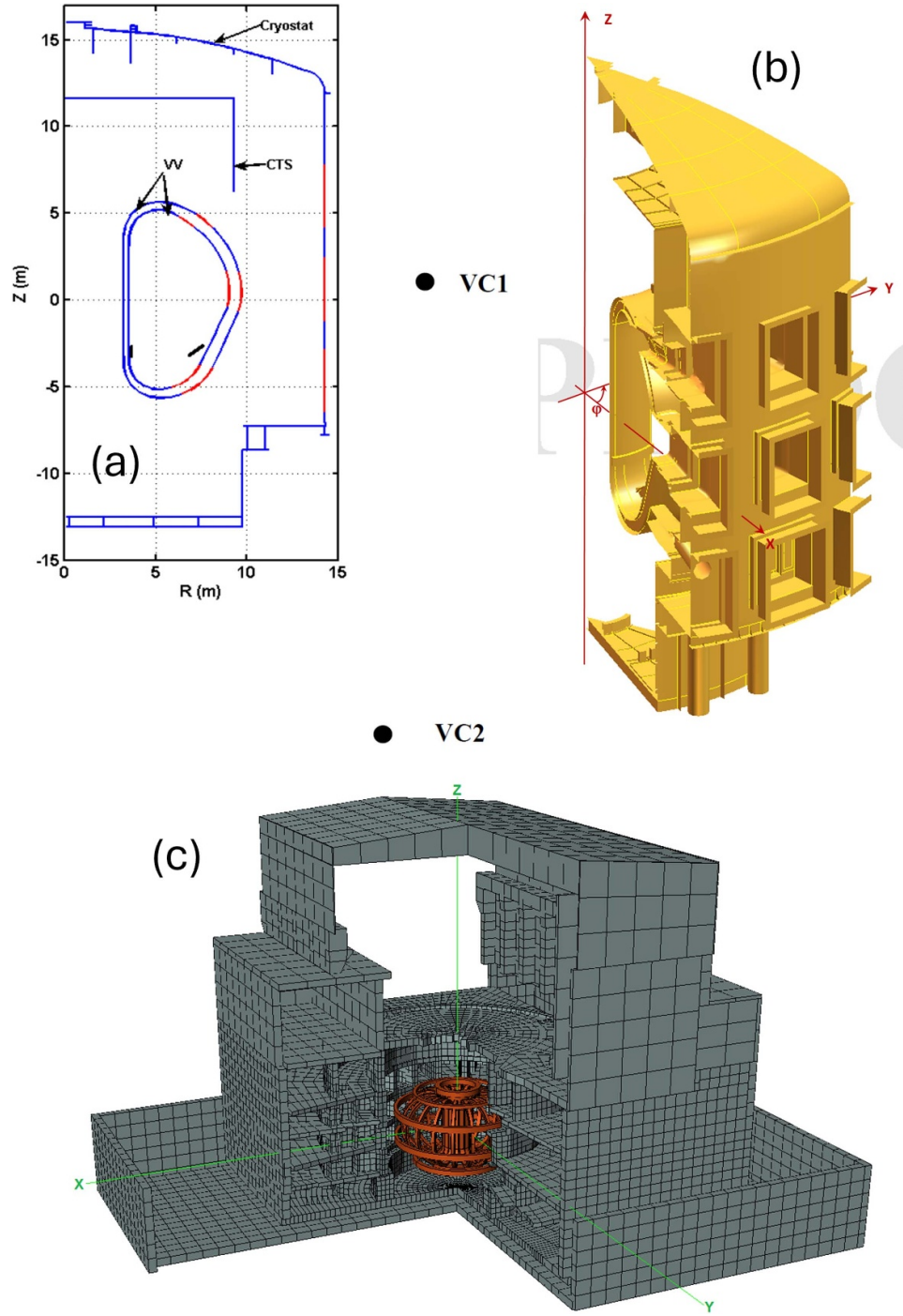
Figure 6. Main elements of Tokamak Electromagnetic Model: (a) 2D models of the vacuum vessel (VV), including toroidally continuous conducting triangular support of blanket modules #18 (vertical black object) and divertor inboard rail (inclined black object), cryostat and cryostat thermal shield (CTS), and virtual coils (VC) with currents reproducing axisymmetric component of magnetic field from ferromagnetic elements of the tokamak buildings, (b) 3D model of the VV, cryostat and CTS, (c) 3D model of ferromagnetic elements of the tokamak building.
