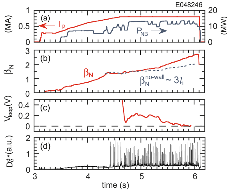
Figure 41. Waveforms of high f_{BS} discharge. (a) Plasma current and NB heating power. (b) Normalized beta and measure of the ideal MHD limit without conducting wall ( \sim 3.0 l_i ). (c) Surface loop voltage. (d) D_{\alpha} intensity at the divertor region. Reproduced from [429]. © 2009 IAEA, Vienna. All rights reserved.
