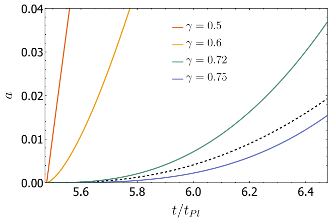
FIG. 4: Outcomes of null geodesics test for \alpha < \bar{\alpha} .
