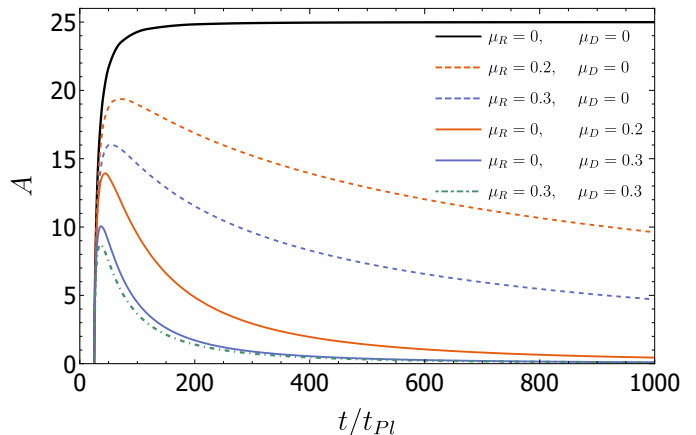
FIG. 2: Anisotropy degree A as a function of t/t_{Pl} for \alpha = -5/3, \mu_I = \sqrt{3}, \mu_A = 0.2\mu_I .
