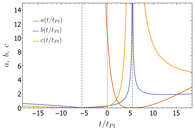
FIG. 3: Numerical solutions as a function of t/t_{Pl} for \mu_I = 0.057 , \mu_A = 2.4 , \mu_D = 0.365 , \mu_R = 1.56 and \alpha = -8.42 < \bar{\alpha} . The dashed lines represent where the scalaron vanishes (color online).
