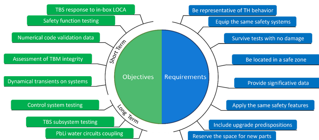
Figure 1. Objectives and requirements of LIFUS5/Mod4 facility.
