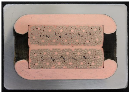
Fig. 6. (Left) Cross-section of the diffusion-bonded joint of two RW cables. Mixed-matrix stabilizer was used in this prototype. (Right) Resistance of the prototype joint as a function of the current and the applied field.
