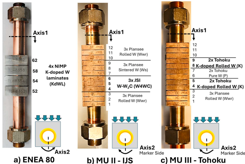
Fig. 1. Inspected mock-ups and measurement axis orientation: a) ENEAS80, a mock-up consisting of 4 K-doped W laminates monoblocks provided by NIMP; b) MU II – IJS, a mock-up containing three W-W 2 C monoblocks provided by IJS; c) MU III – Tohoku, equipped with four K-doped rolled W monoblocks.
