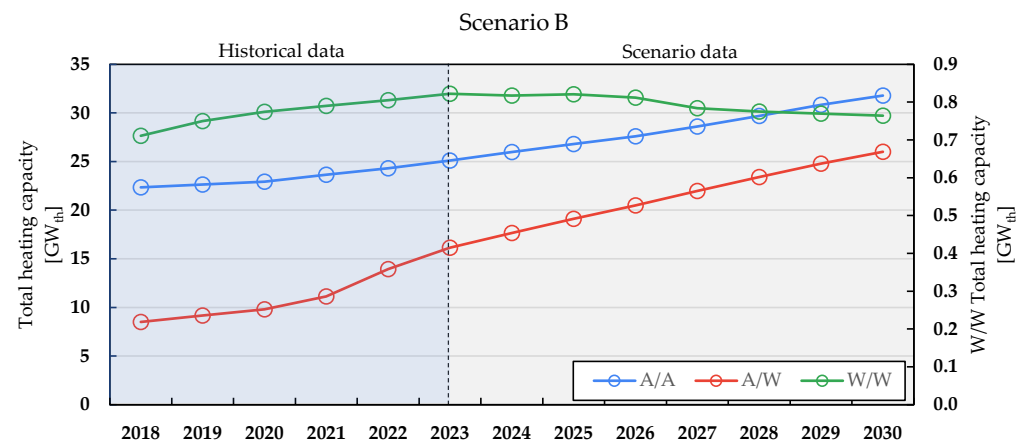
Figure 8. Evolution of total heating capacity in Scenario B.
