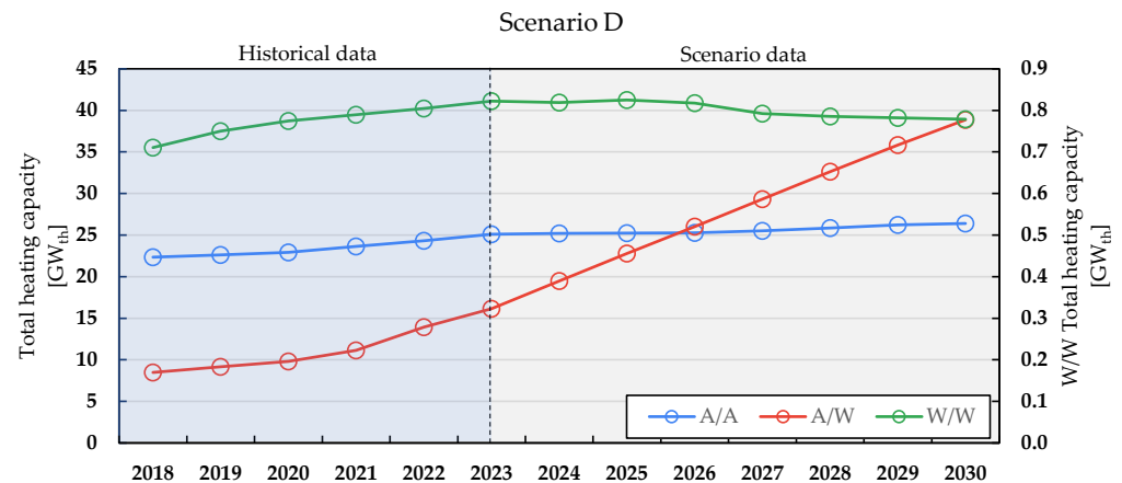
Figure 10. Evolution of total heating capacity in Scenario D.
