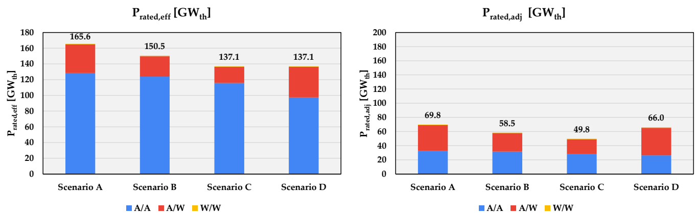
Figure 5. Total thermal capacity in the considered scenarios.
