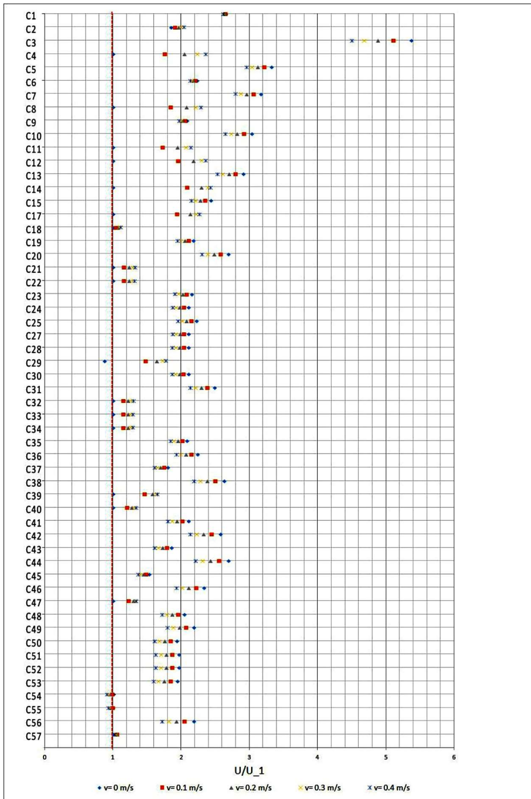
Figure 3. U-value ratios at different wind speed using Equation 1.
