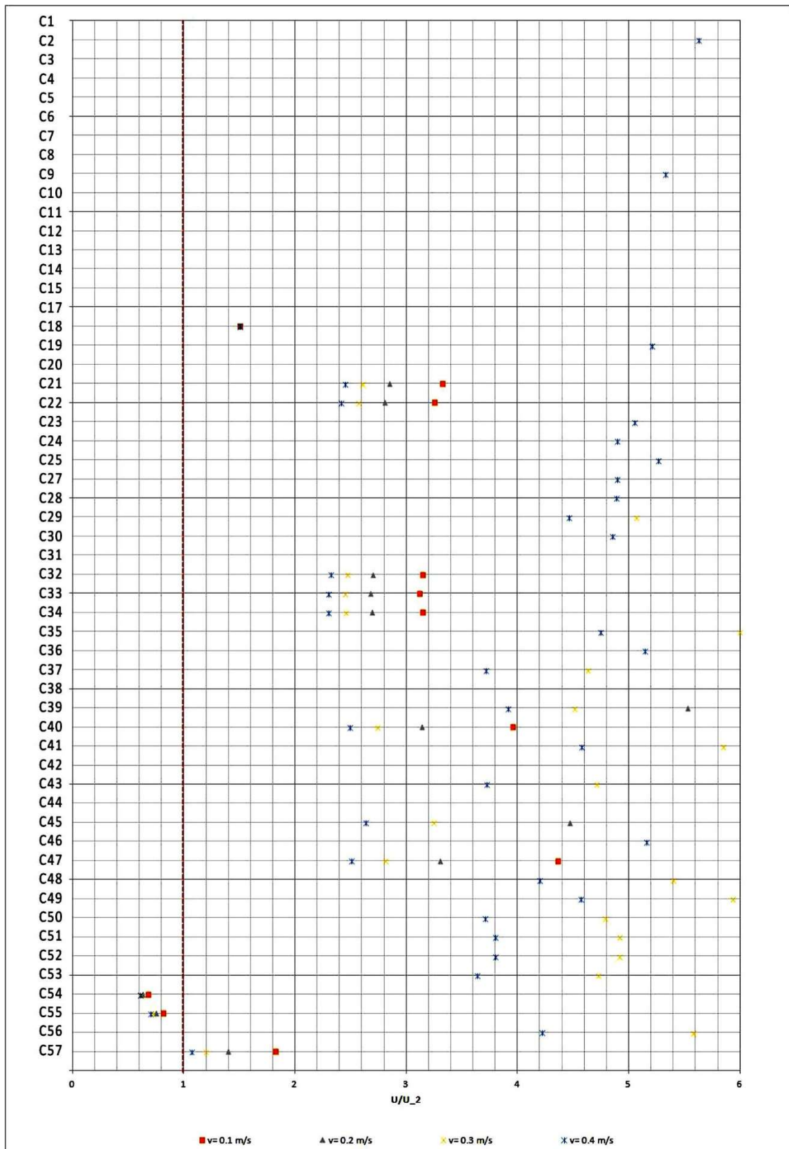
Figure 5. U-value ratios at different wind speed using Equation 2 – detail of the ratio range 0-6.
