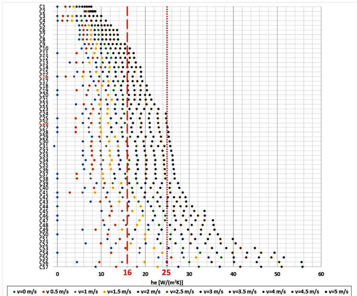
Figure 2. CHTC comparison for wind speed ranging between 0 m/s and 5 m/s.
