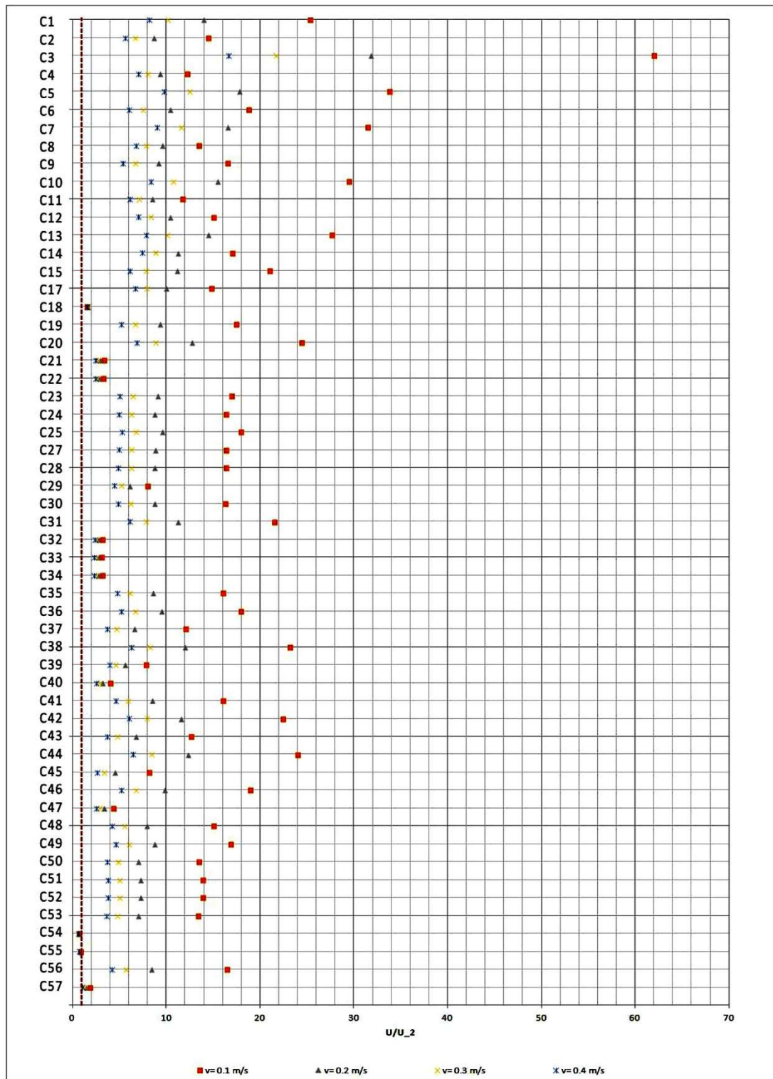
Figure 4. U-value ratios at different wind speed using Equation 2.
