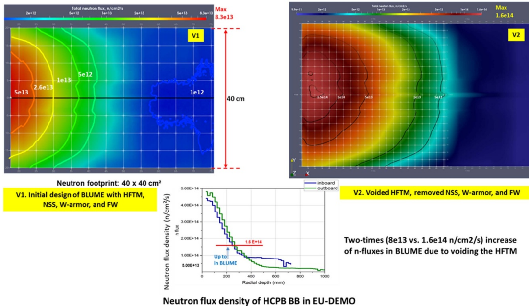
Figure 12. Relevance of neutron flux ( n\text{ cm}^{-2}\text{ s}^{-1} ) in BLUME-1 to the values in the breeding zone of the DEMO HCPB breeding blanket. Reproduced from [28]. © 2025 The Author(s). Published by IOP Publishing Ltd on behalf of the IAEA. CC BY 4.0.
