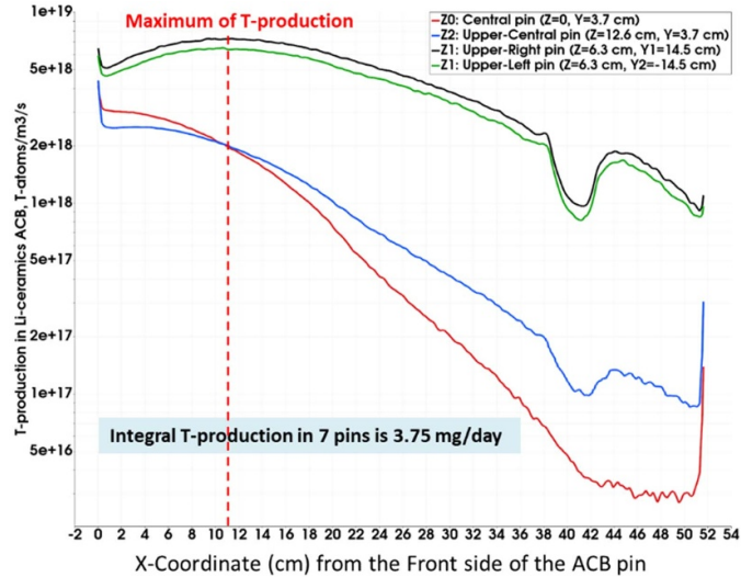
Figure 20. 1D profiles of T-production rate ( T \text{ m}^{-3} \text{ s}^{-1} ) in the ACB with 90 at% of {}^6\text{Li} enrichment, BLUME-7 with C-reflector.
