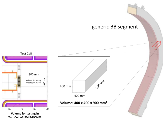
Figure 6. Schematics that conceptually shows the idea of the TBU and the available volume for testing breeder/multiplier in the test cell.
