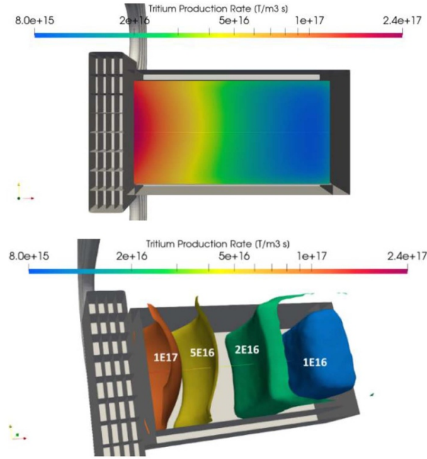
Figure 23. Tritium production rate ( T\ m^{-3}\ s^{-1} ) map in the WCLL-TBU, lateral cross section of 30 \times 30\ cm^2 . (a) Horizontal cross section ( z = 0 ); (b) contour surfaces.
