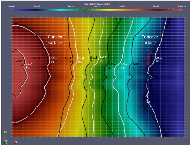
Figure 18. 2D horizontal ( x - y ) central cut of the 3D map neutron flux ( n \text{ cm}^{-2} \text{ s}^{-1} ) in depth distribution of BLUME-7 shown in figure 17.
