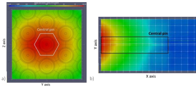
Figure 14. Transversal gradients of the nuclear (neutrons and photons) heat density (W cm -3 ) in single material TiBe12 of BLUME-1 (a) vertical cut and (b) horizontal cut.
