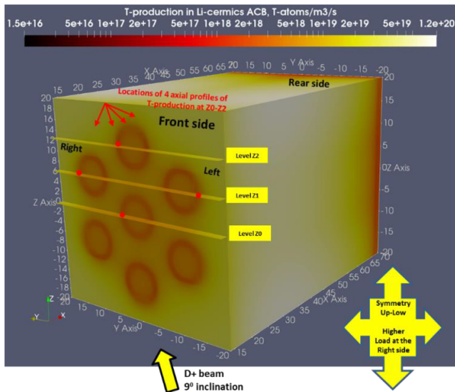
Figure 19. 3D map of T-production ( T \text{ m}^{-3} \text{ s}^{-1} ) in ACB with 90 at% of {}^6\text{Li} enrichment, calculated in BLUME-7 with graphite reflector.
