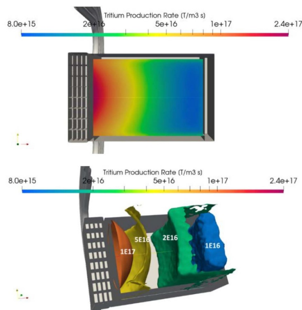
Figure 22. Tritium production rate ( T\ m^{-3}\ s^{-1} ) map in the WCLL-TBU, lateral cross section of 40 \times 40\ cm^2 . (a) Horizontal cross section ( z = 0 ); (b) contour surfaces.
