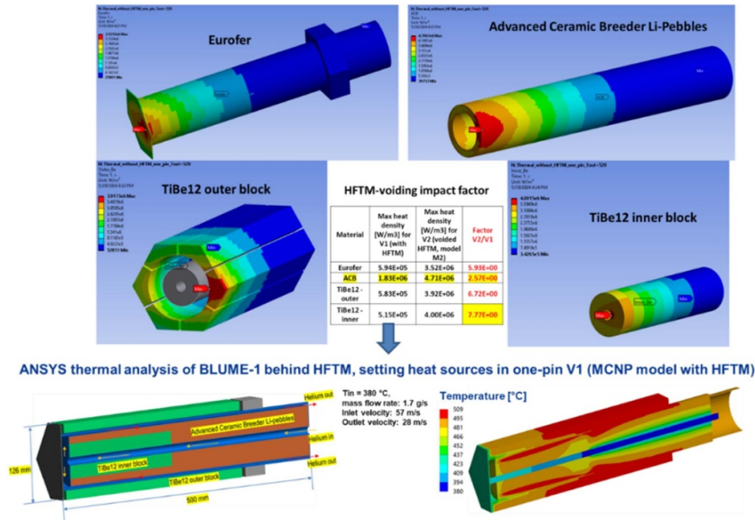
Figure 13. 3D distributions of the MCNP results of heat density (W m -3 ) sources (neutrons and photons) calculated in three materials (EUROFER, ACB, and TiBe12) of the BLUME-1 V1 model with HFTM set in the CAD-coupled ANSYS model and produced temperature (°C) distribution by following the CAD-based integrated neutronic-thermomechanical modeling [40]. Reproduced from [28]. © 2025 The Author(s). Published by IOP Publishing Ltd on behalf of the IAEA. CC BY 4.0.
