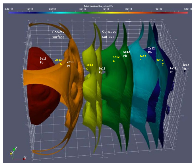
Figure 17. 3D map of the neutron flux ( n \cdot cm^{-2} \cdot s^{-1} ) distribution in depth of the BLUME-7 model.
