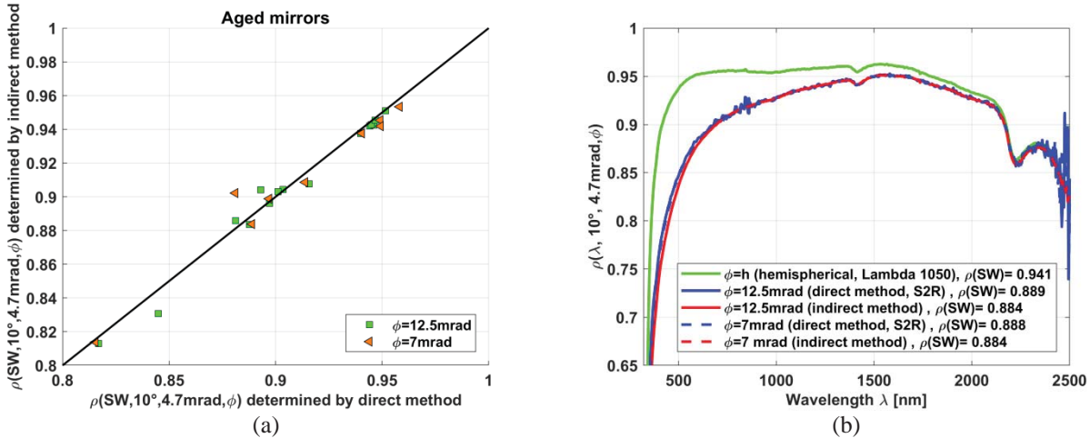
FIGURE 4. Comparison of the direct and indirect methods for outdoor aged mirror samples (a) Solar-weighted near-normal sun-conic reflectance at \varphi=\{7, 12.5\} mrad of 17 mirror samples. (b) Spectral near-normal sun-conic reflectance at \varphi=\{7, 12.5\} mrad for one of the 17 measured mirror samples.
