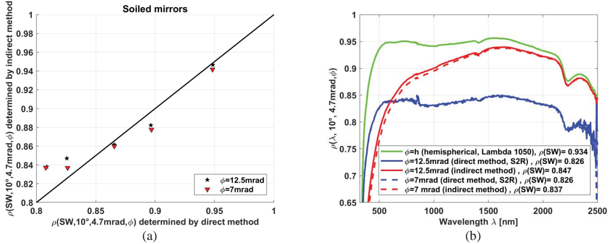
FIGURE 5. Comparison of the direct and indirect methods for soiled mirror samples (a) Solar-weighted near-normal sun-conic reflectance at \phi=\{7, 12.5\} mrad of 5 mirror samples. (b) Spectral near-normal sun-conic reflectance at \phi=\{7, 12.5\} mrad for one of the 5 measured mirror samples.
