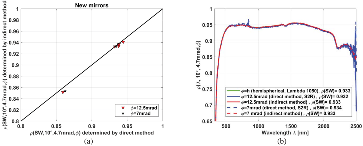
FIGURE 3. Comparison of the direct and indirect methods for new mirror samples (a) Solar-weighted near-normal sun-conic reflectance at \varphi=\{7, 12.5\} mrad of 5 new mirror samples. (b) Spectral near-normal sun-conic reflectance at \varphi=\{7, 12.5\} mrad for one of the 5 measured mirror samples.
