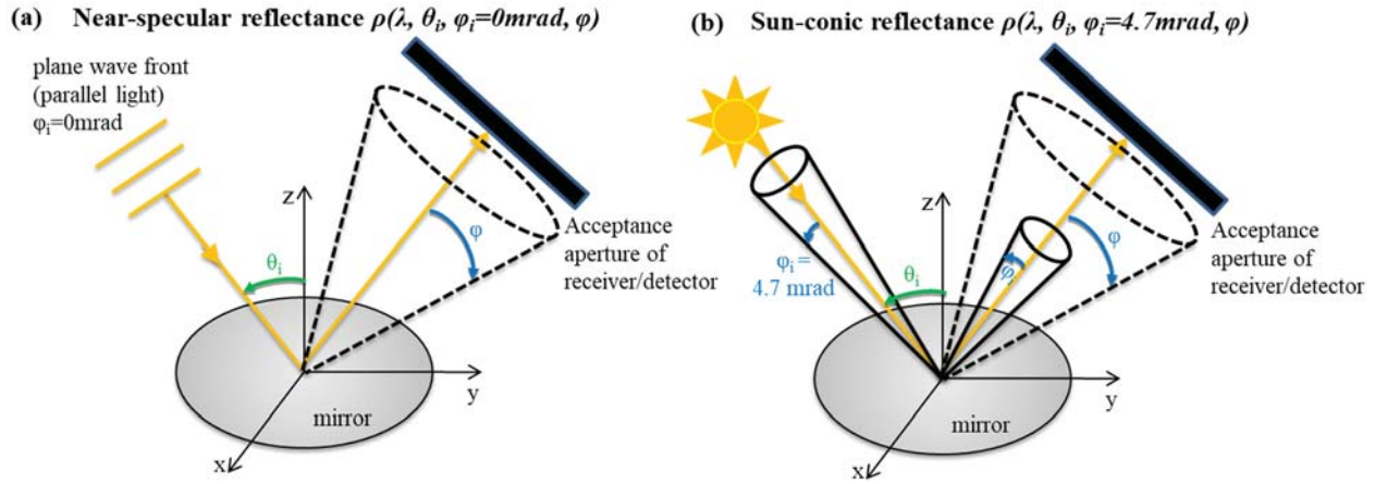
FIGURE 1 Illustration of reflectance parameters. The incidence angle is \theta_i , the acceptance angle of the solar receiver or detector is \varphi . (a) Near-specular reflectance, the beam divergence of the impinging light source is \varphi_i = 0 mrad. (b) Sun-conic reflectance, the beam divergence of the solar disc is \varphi_i = 4.7 mrad.
