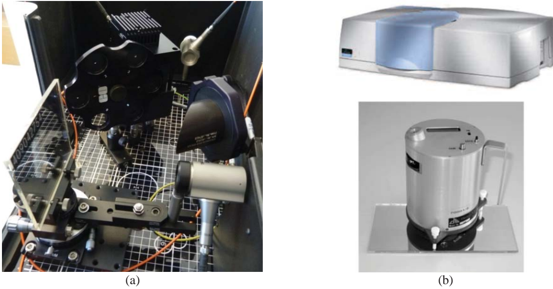
FIGURE 2. Employed equipment to determine solar-weighted near-normal sun-conic reflectance at \varphi = \{7, 12.5\} mrad. (a) Spectral Specular Reflectometer S2R used for the direct method, (b) Perkin Elmer Lambda 1050 spectrophotometer and D&S 15R-USB reflectometer for the indirect method.
